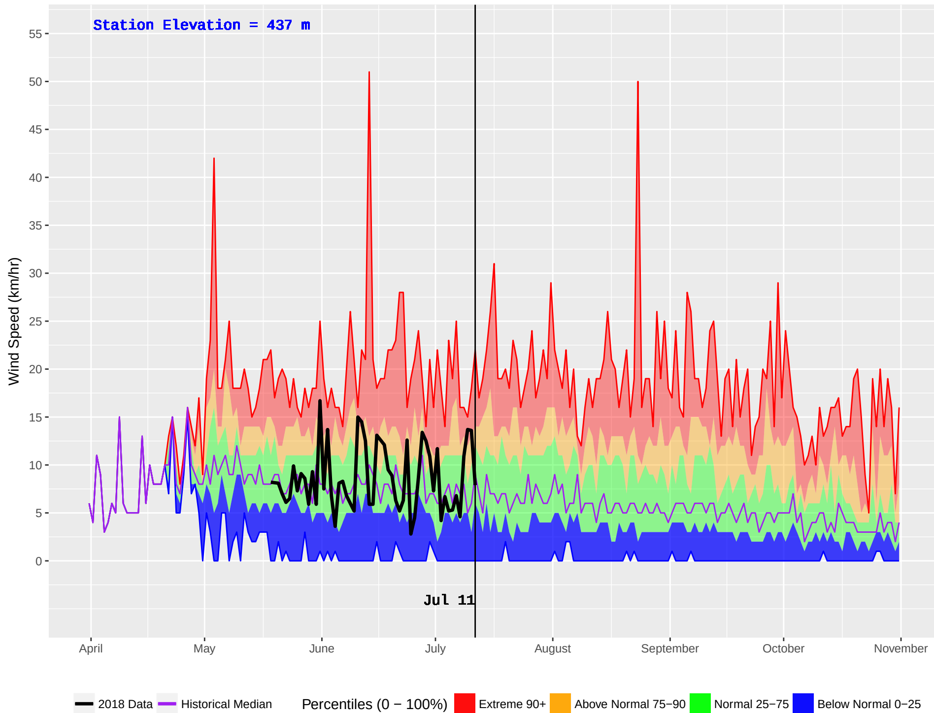
ELK MOUNTAIN (438) : Historical (1973–2016) and Current (2018) Noon Wind Speed
