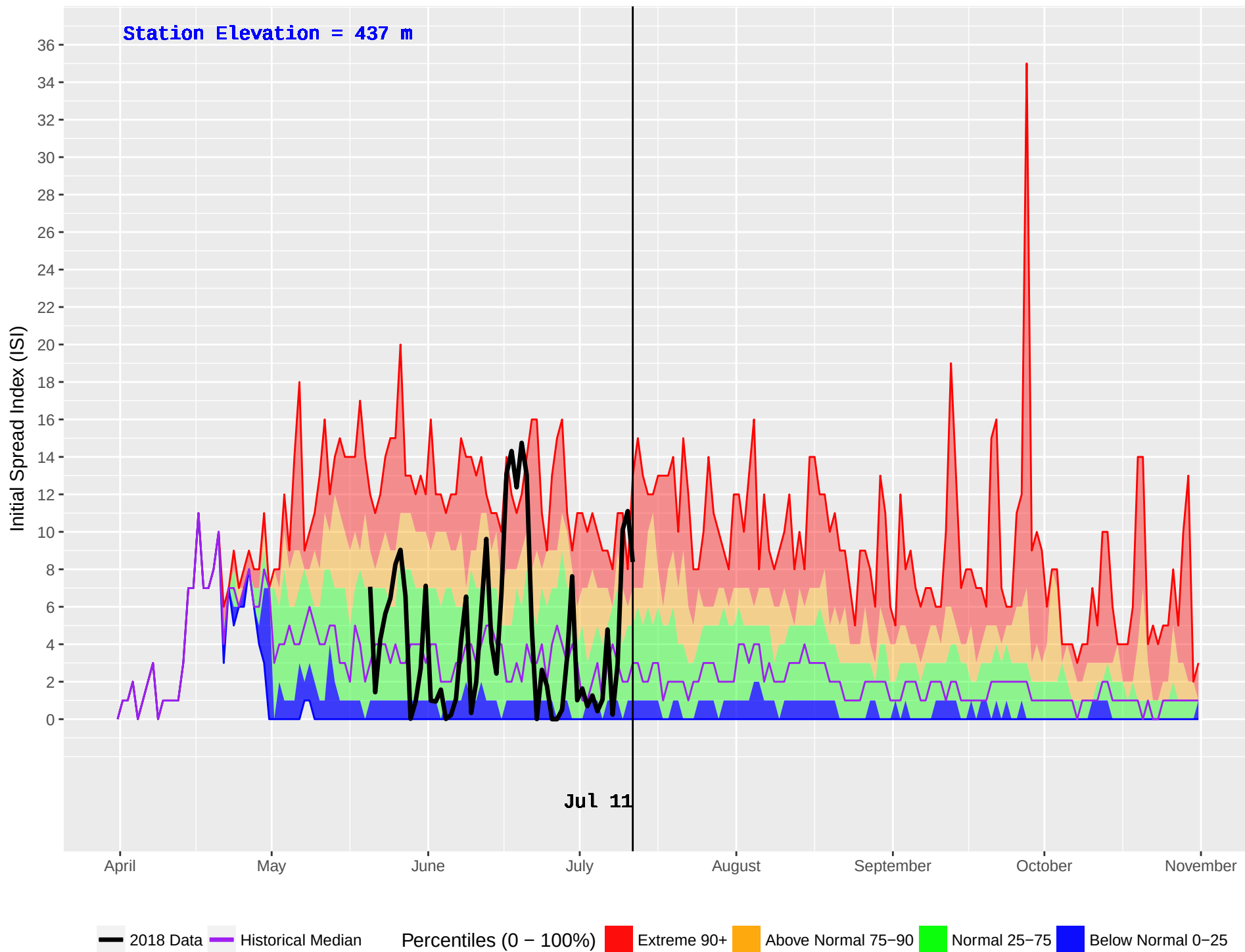
ELK MOUNTAIN (438) : Historical (1973–2016) and Current (2018) Noon Initial Spread Index (ISI)
