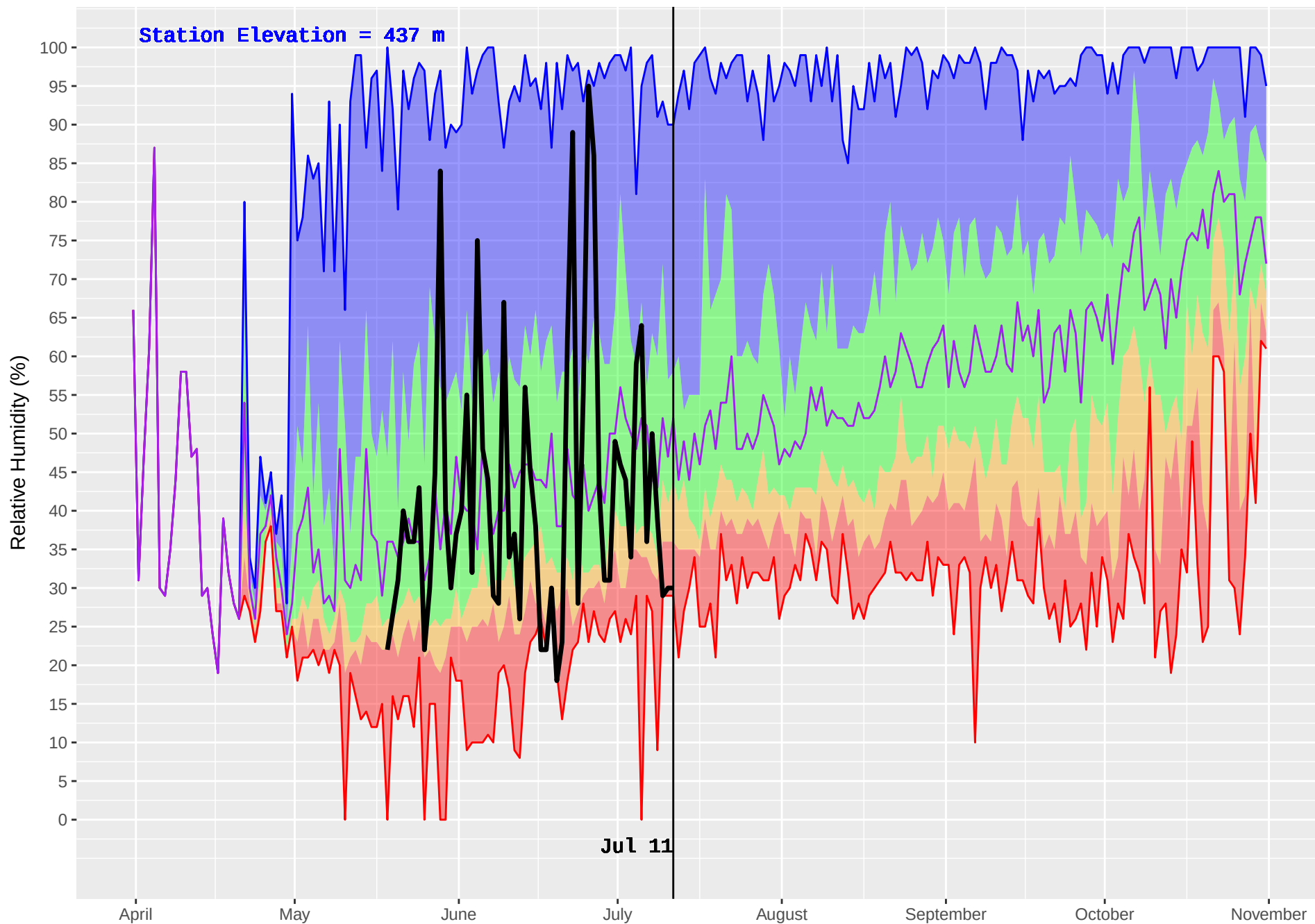
ELK MOUNTAIN (438) : Historical (1973–2016) and Current (2018) Noon Relative Humidity
