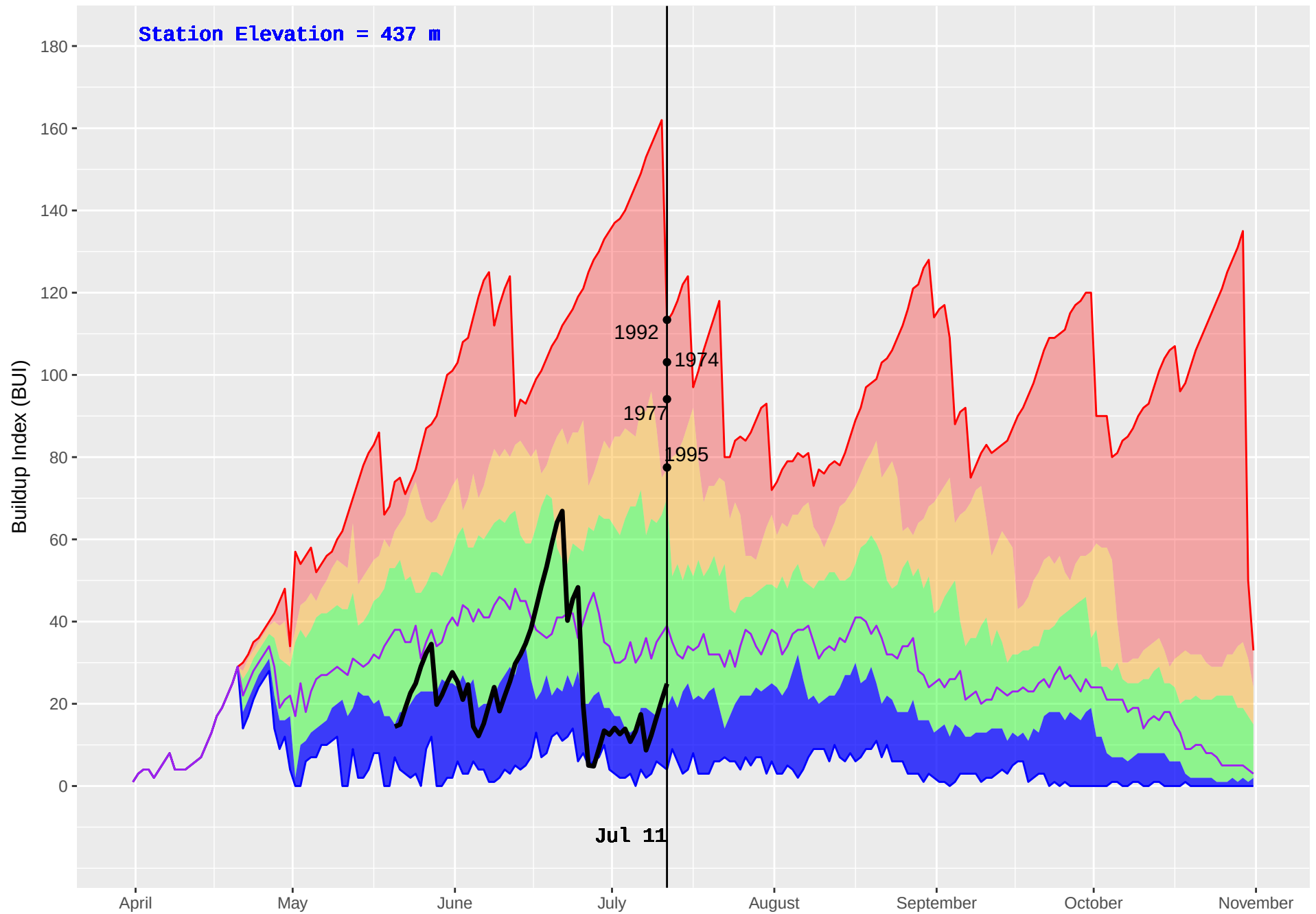
ELK MOUNTAIN (438) : Historical (1973–2016) and Current (2018) Noon Buildup Index (BUI)
