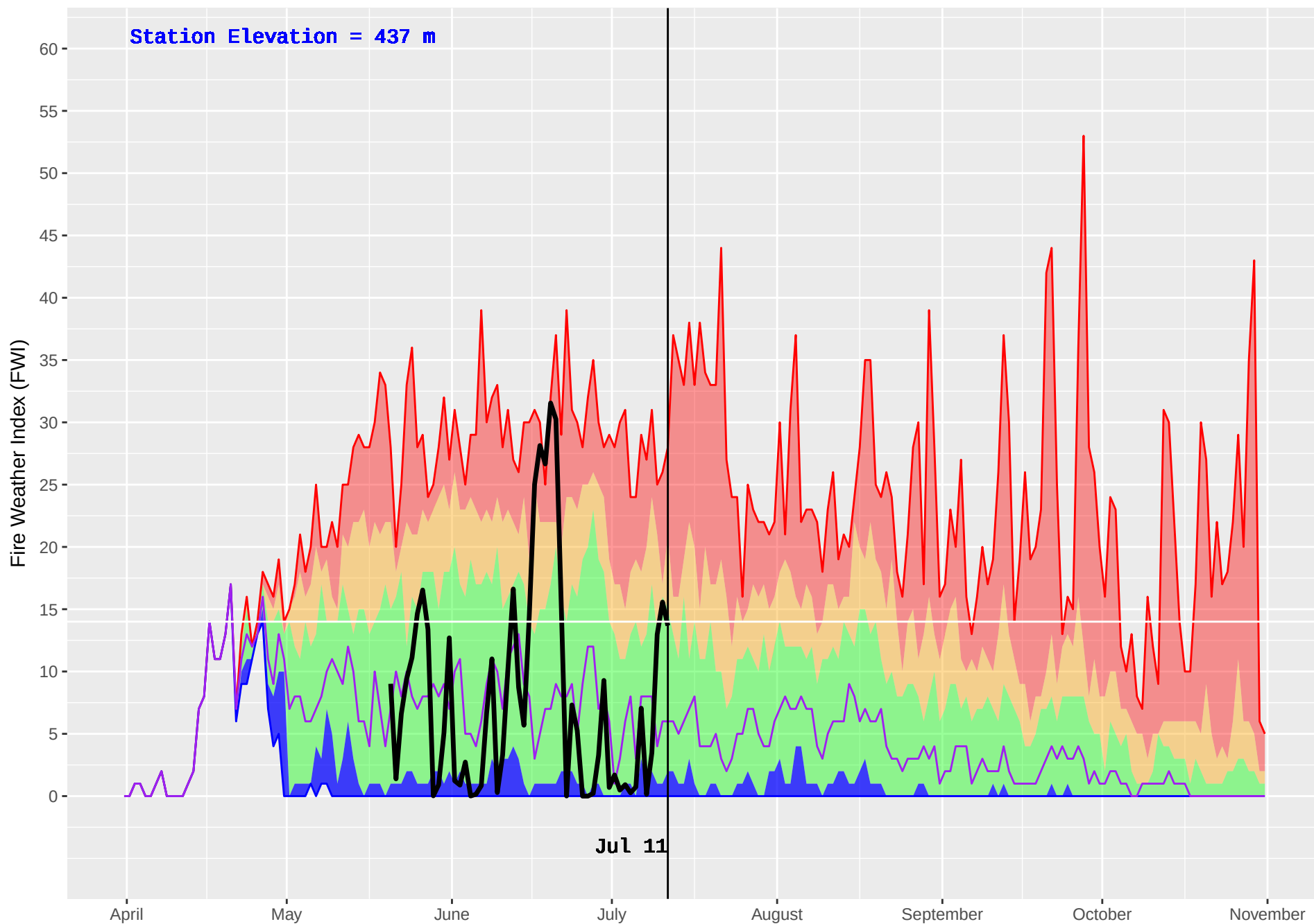
ELK MOUNTAIN (438) : Historical (1973–2016) and Current (2018) Noon Fire Weather Index (FWI)
